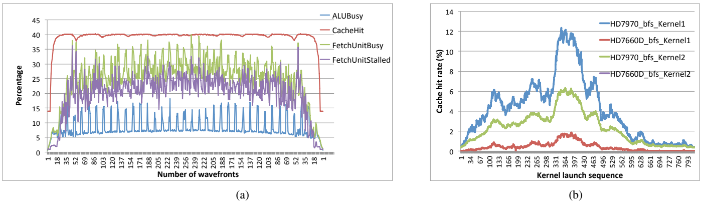
Fig. 6: (a) NW profiling on HD7660D. (b) BFS cache performance comparison between HD7970 and HD7660D.
